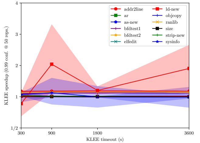
Figure 9: Speedup when executing 17 Binutils tools. The legend shows those tools with the highest and lowest speedup. We observe that the variance is significantly higher than for the Coreutils experiments and PARTI achieves little to no overall speedup.
