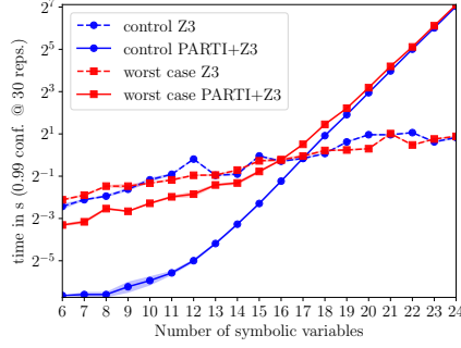
Figure 4: Runtime for the symbolic execution of the worst case and control programs (cf. §4.1.2). PARTI performs well for up to 16 Add expressions. Afterwards the exponential blowup due to additions in the decision stage take over.
